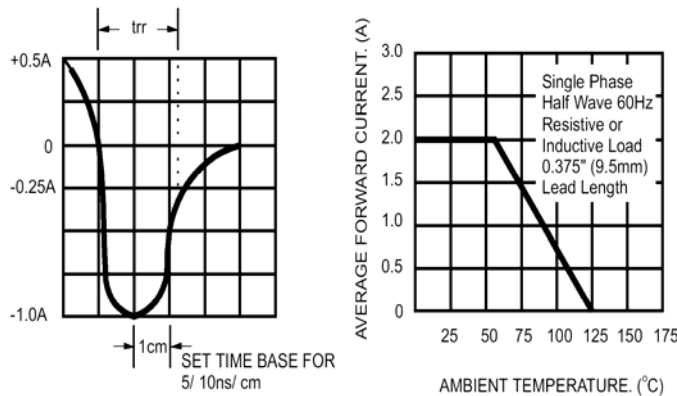
FIG.2- MAXIMUM AVERAGE FORWARD CURRENT DERATING
