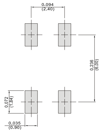
FIG.6 MOUNTING PAD LAYOUT
