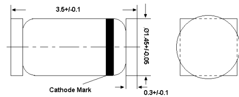
Glass case QuadroMELF Dimensions in mm
